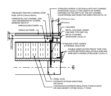
8 WINDOW AND DOOR JAMB (CAULKING) (STEEL STUD)
