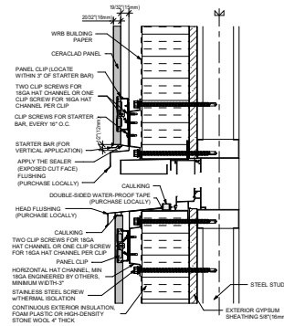
8 WINDOW AND DOOR HEAD AND SILL (CAULKING)
