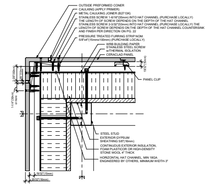
4 OUT SIDE PREFORMED CORNER (STEEL STUD)
