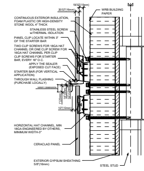
7 THROUGH WALL FLASHING (STEEL STUD)
