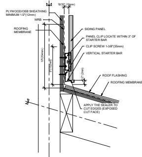
9 ROOF TO WALL (STEEL STUD)
