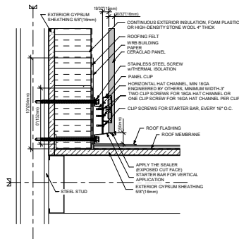
9 LOW SLOPE ROOF AND WALL (STEEL STUD)
