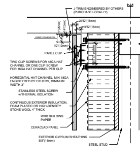
6 UNDER EAVES (STEEL STUD)
