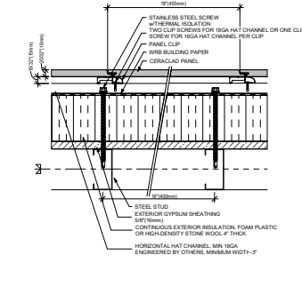
2 PANEL VERTICAL JOINT (HORIZONTAL SECTION)
