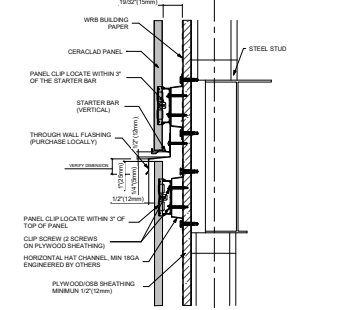
7 THROUGH WALL FLASHING (STEEL STUD)
