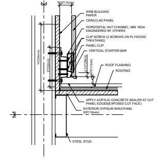
9 LOW SLOPE ROOF AND WALL (STEEL STUD)
