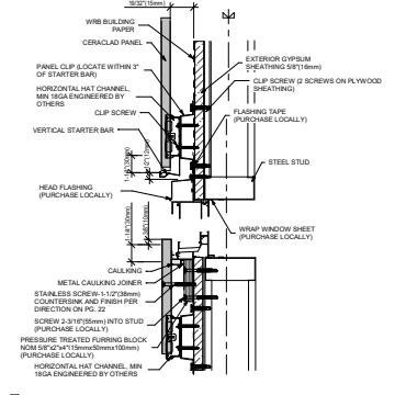
8 WINDOW AND DOOR HEAD AND SILL (STEEL STUD)
