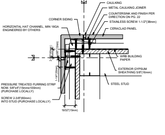
4 OUT SIDE PREFORMED CORNER (STEEL STUD)
