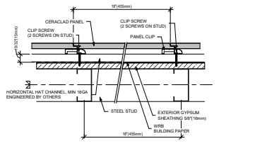
2 PANEL VERTICAL JOINT (HORIZONTAL SECTION)
