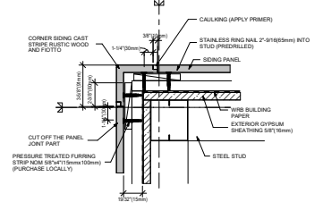
4 OUT SIDE PREFORMED CORNER A (STEEL STUD)
