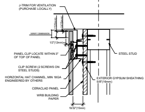
6 UNDER EAVES (STEEL STUD)
