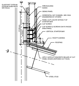
9 ROOF TO WALL (STEEL STUD)
