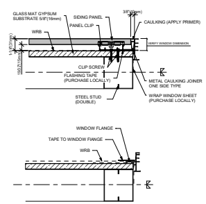
8 WINDOW AND DOOR JAMB (CAULKING) (STEEL STUD)
