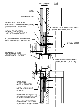
8 WINDOW AND DOOR HEAD AND SILL (CAULKING)
