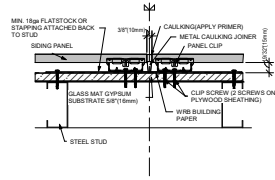
3 PANEL CAULKING JOINT (STEEL STUD)
