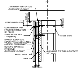
6 UNDER EAVES (STEEL STUD)
