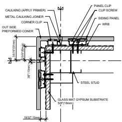
4 OUTSIDE METAL CORNER (STEEL STUD)
