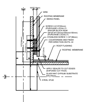
9 LOW SLOPE ROOF AND WALL (STEEL STUD)
