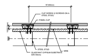
2 HORIZONTAL JOINT (STEEL STUD)
