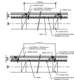
2 PANEL VERTICAL JOINT
