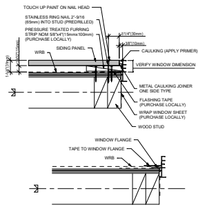
8 WINDOW AND DOOR JAMB (CAULKING)
