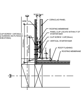
9 LOW SLOPE ROOF AND WALL
