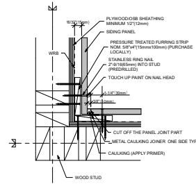
5 INSIDE CORNER
