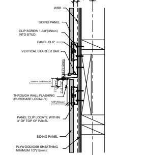
7 THROUGH WALL FLASHING
