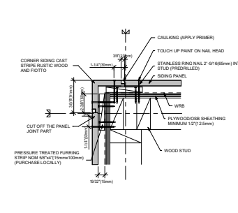
4 OUTSIDE PREFORMED CORNER A
