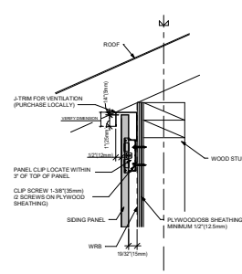
6 UNDER EAVES
