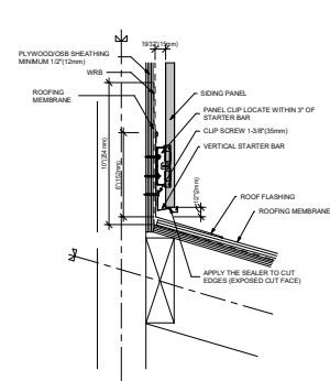
9 ROOF TO WALL
