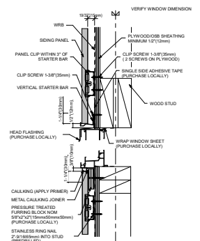
8 WINDOW AND DOOR HEAD AND SILL (CAULKING)
