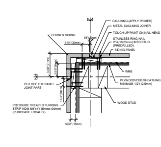
4 OUTSIDE PREFORMED CORNER
