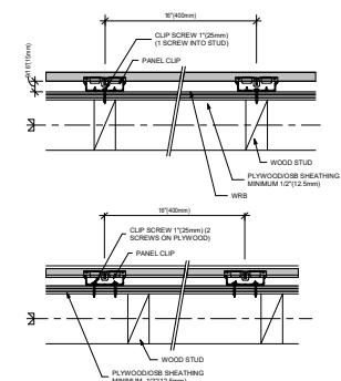
2 HORIZONTAL PANEL JOINT
