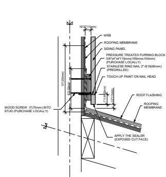
9 ROOF to WALL (Wood frame)
