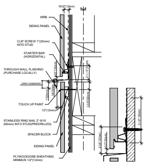
7 THROUGH WALL FLASHING
