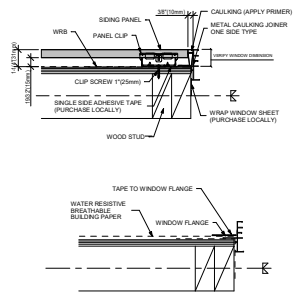
8 WINDOW AND DOOR JAMB (CAULKING)
