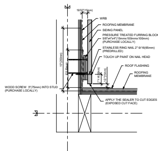
9 TERMINATION ABOVE ROOF
