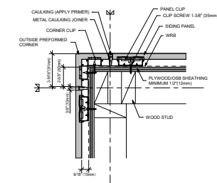
4 OUTSIDE CORNER - 18" PREFORMED CORNER
