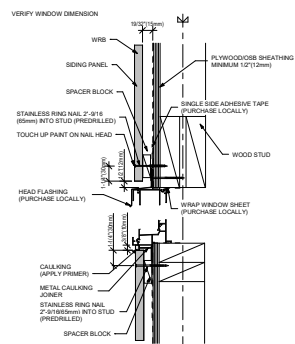
8 WINDOW AND DOOR HEAD AND SILL(CAULKING)
