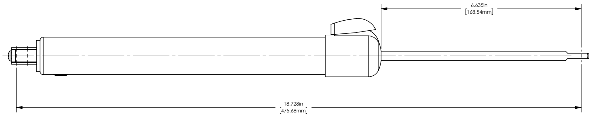
MAX EXTENDED POSITION MAX DOOR OPENING ANGLE 77°
