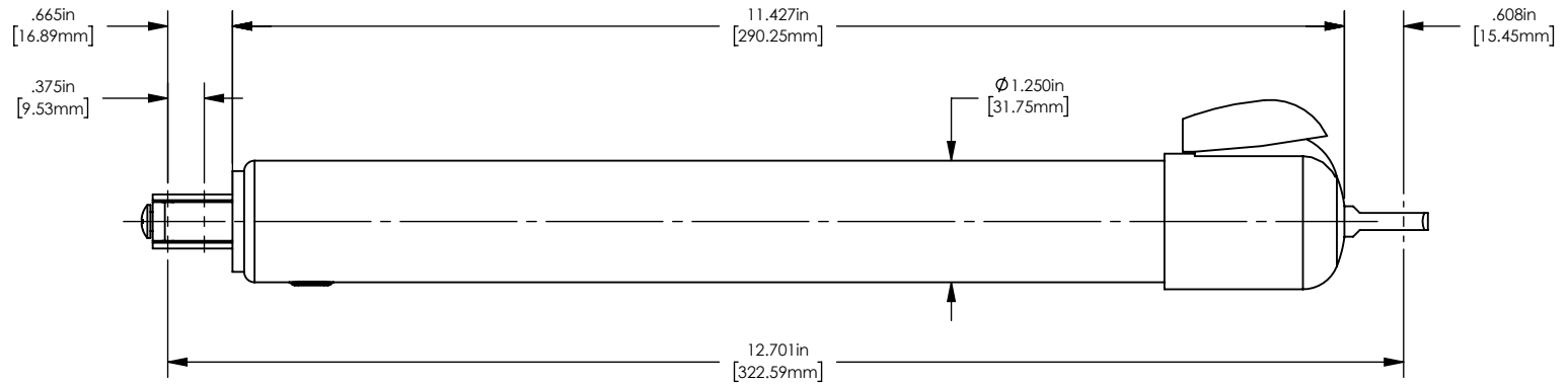
INSTALLED POSITION
