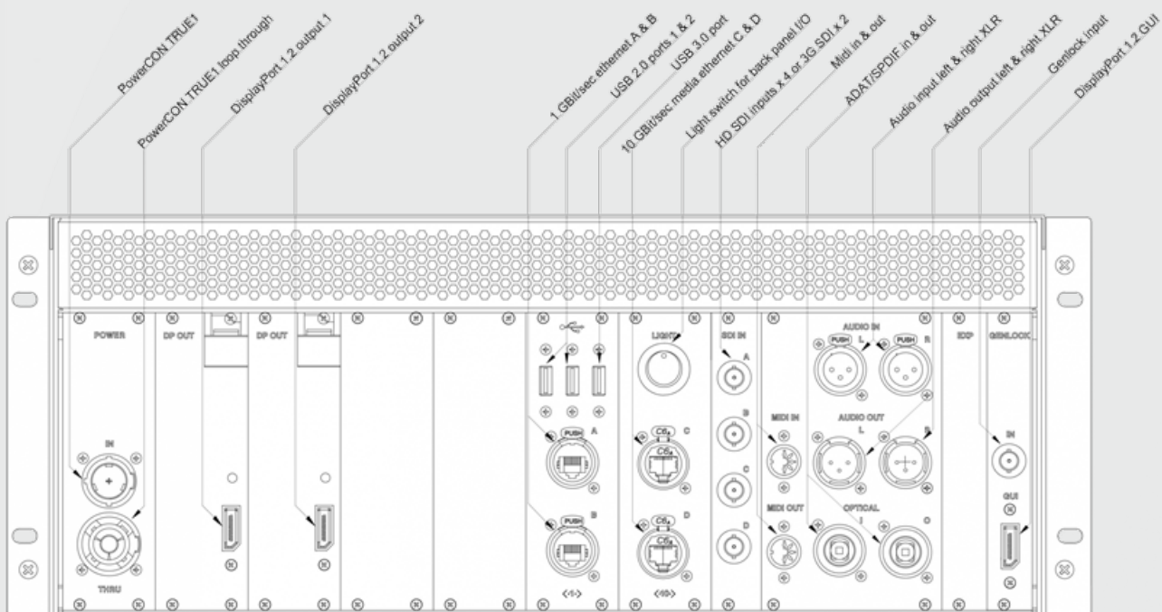
gx 2 rear panel annotated
