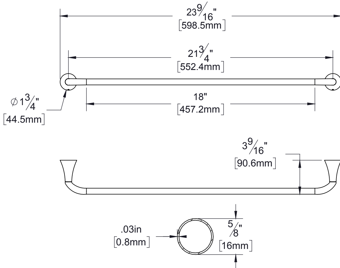
TOWEL BAR CROSS SECTION
