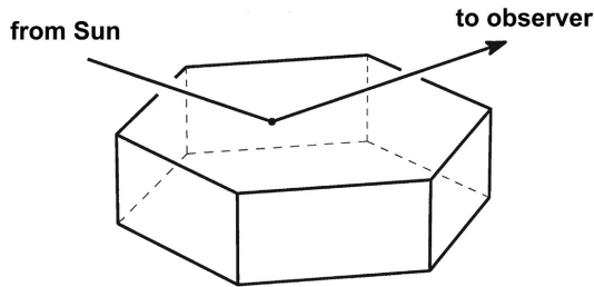
Fig. 1. A subsun arises from preferentially oriented ice crystals with at least one of its faces horizontally oriented. In most cases, the subsun-generating crystals are hexagonal plates, oriented as depicted in this diagram. External reflection of Sun light at the horizontally oriented upper face creates a subsun.
