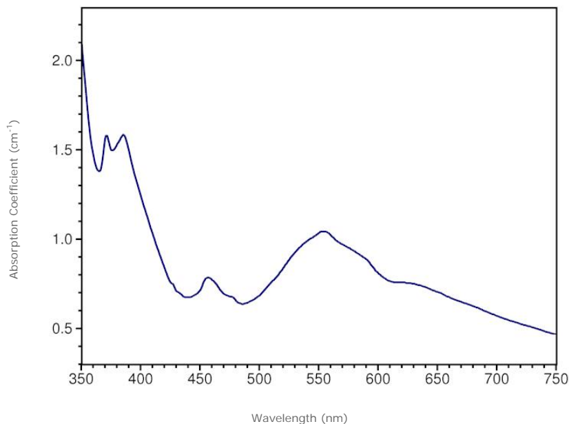
Visible Absorption | min. path length: 6.1 mm
