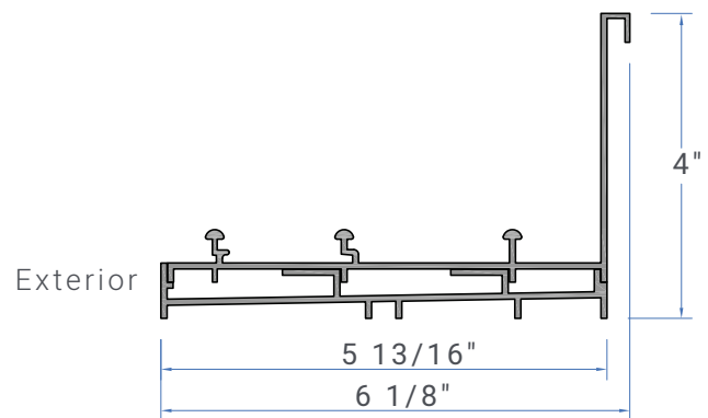
Frame sill reinforced sliding door
