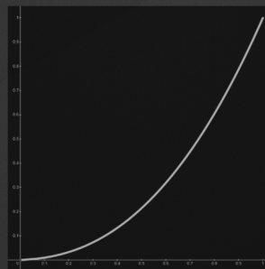
CRT's EOTF
