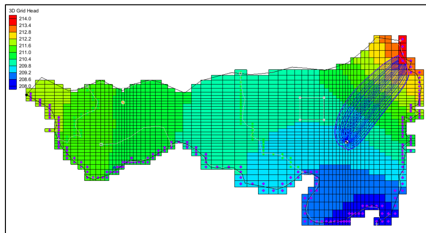
Figure 2 After west well pathlines and particles are deleted
