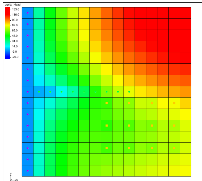
Figure 9 Contours of MODFLOW 6 solution
