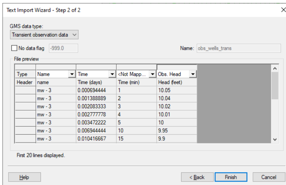
Figure 7 Step 2 of the Text Import Wizard
