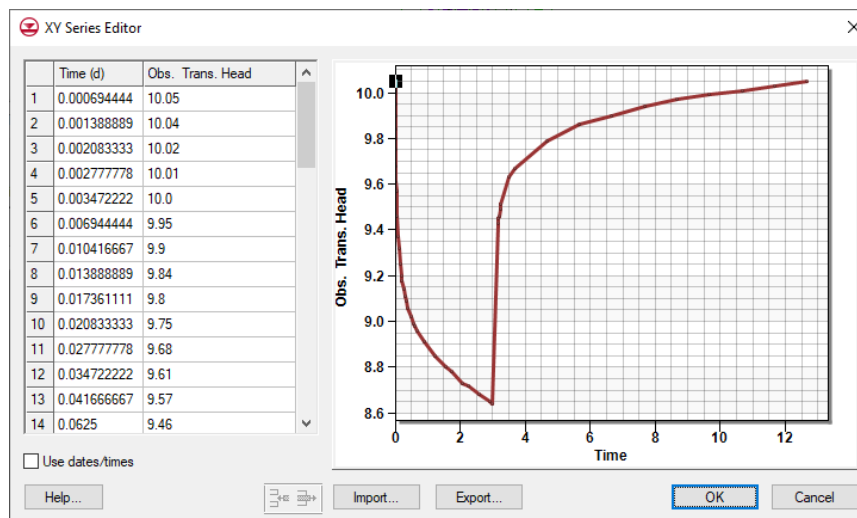
Figure 8 Time series data for well “mw - 3”
