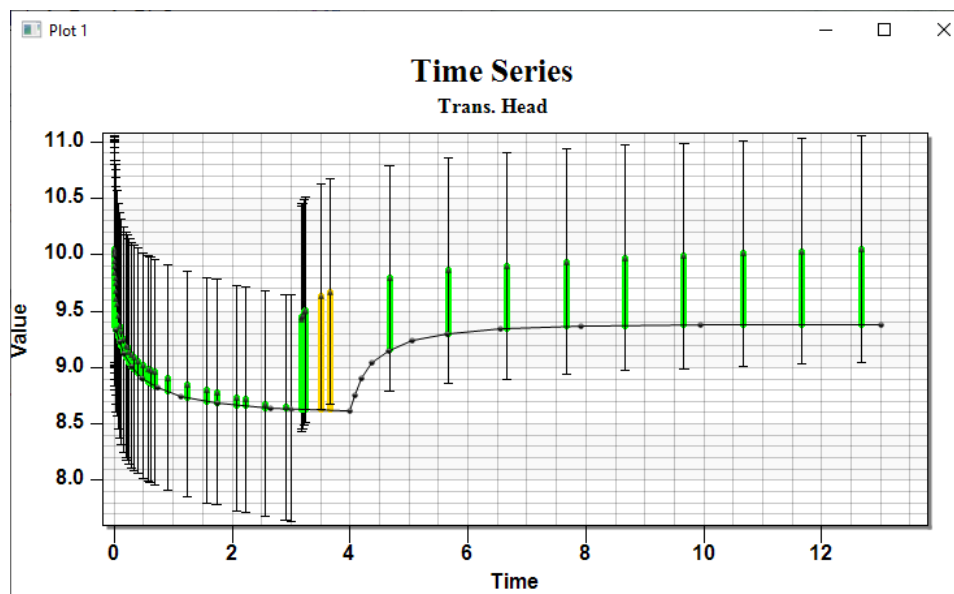
Figure 12 Time series Plot after PEST Calibration
