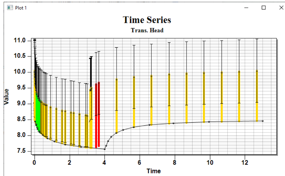
Figure 11 Time series plot after PEST run
