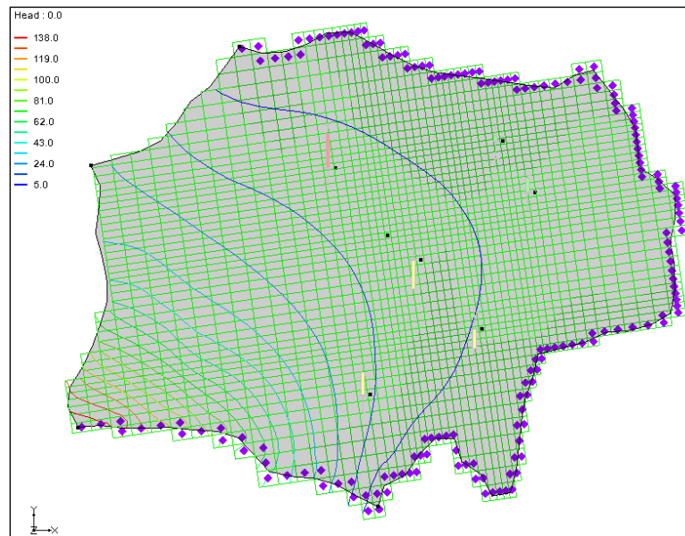
Figure 9 The contours changed slightly after running MODFLOW
