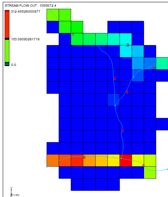
Figure 13 Stream Reach Flow
