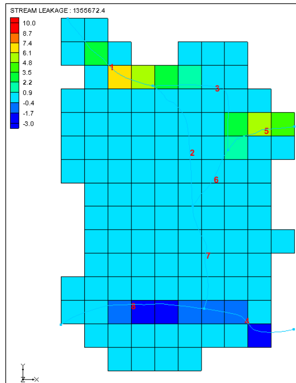
Figure 12 Block Fill showing stream in/out flow
