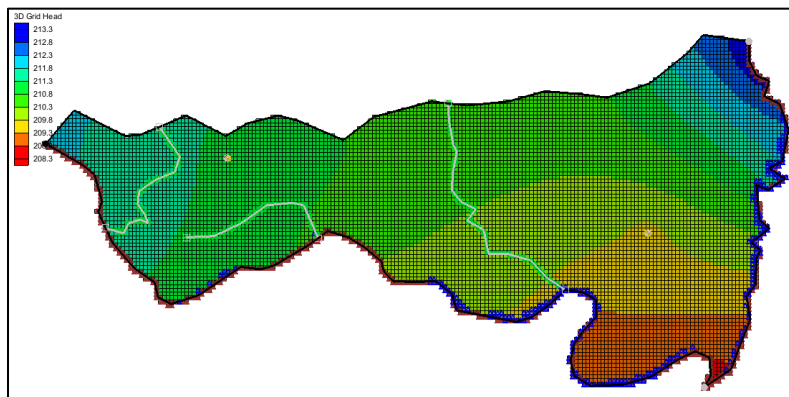
Figure 8 Contours of layer 1 after the model run
