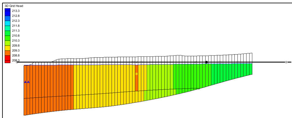
Figure 9 Side view of the model
