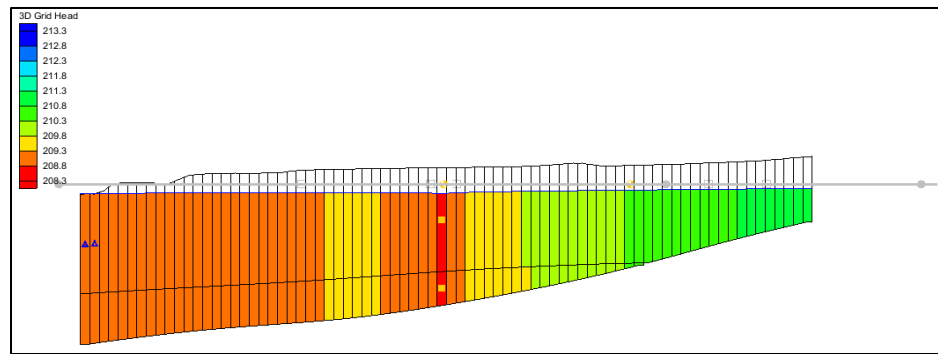
Figure 10 Side view of the model with well depression visible
