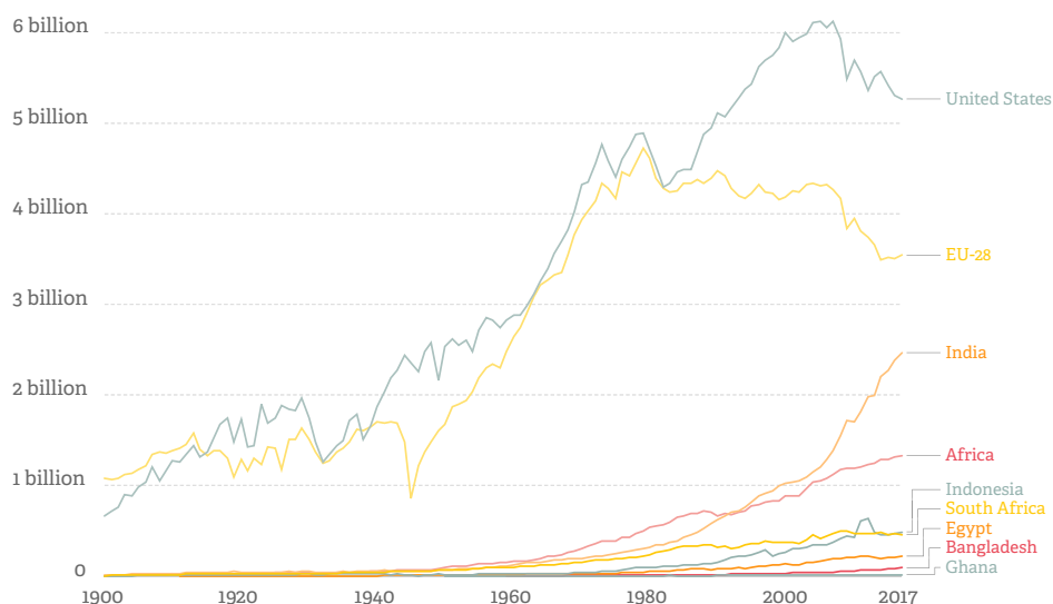
Figure 2: Annual carbon dioxide emissions by country/region (tonnes per year) (Source: Our World in Data, 2018 (from Global Carbon Project, Carbon Dioxide Information Analysis Centre))
