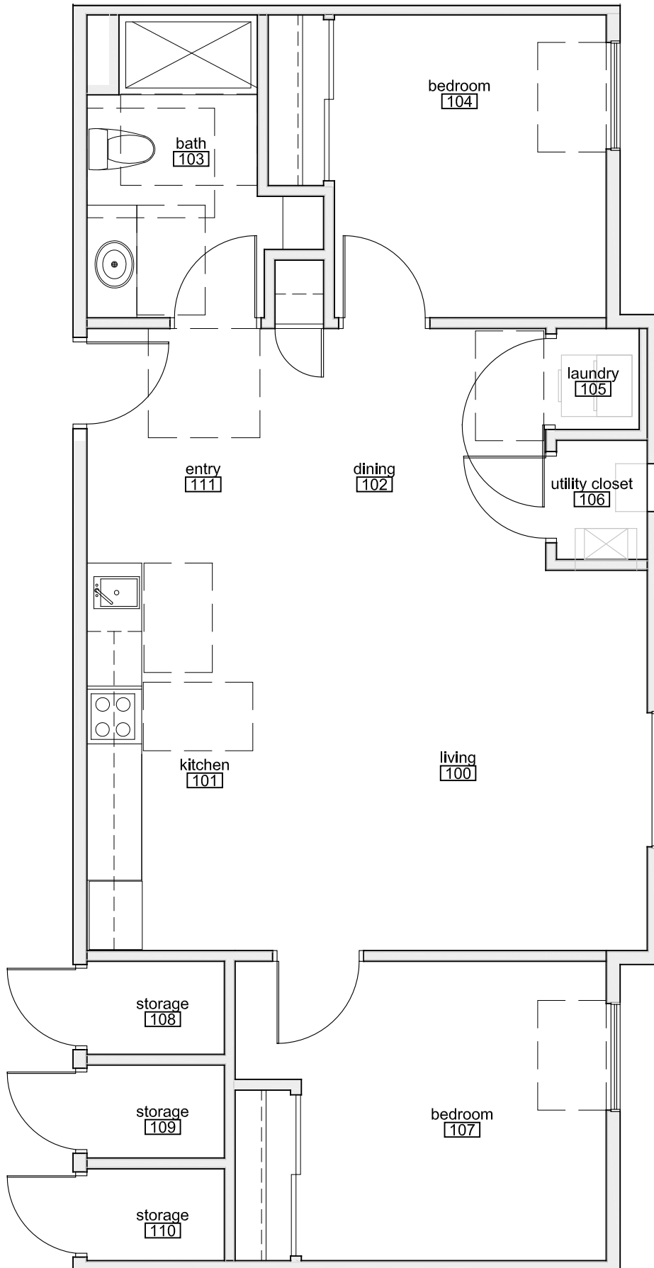
enlarged unit plan type A3 - type B
