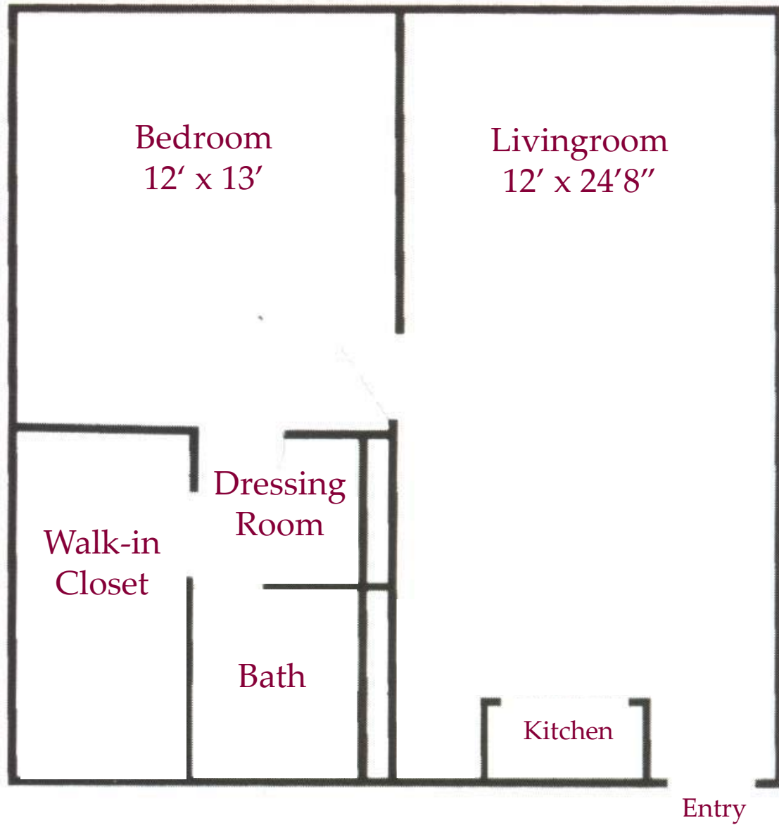
Sun City Gardens Plan A - One Bedroom/One Bath 594 Sq. Ft.
