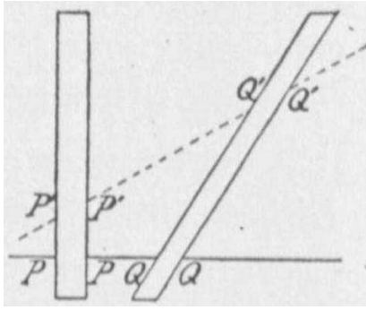
Figure 1: In Minkowski's paper "Space and Time" Fig. 1, which is reproduced here, represents two Lorentzian electrons by their worldtubes or as Minkowski called them "world bands".
