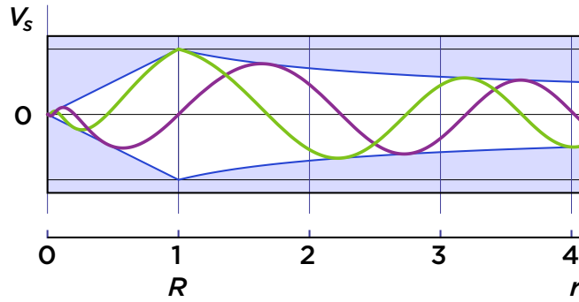
Fig. 1 Inspired by L. C. Epstein’s tubular modeling of GR, [6] the Rotonian tubular model—whose cross-section is shown here—differs markedly, first of all, because it moves . Epstein’s model was designed to accommodate the static block time picture and to represent motion through space, as frozen paths on a curled up spacetime diagram. The Rotonian model represents motion of space—into or outfrom a fourth spatial dimension. (See text.)
