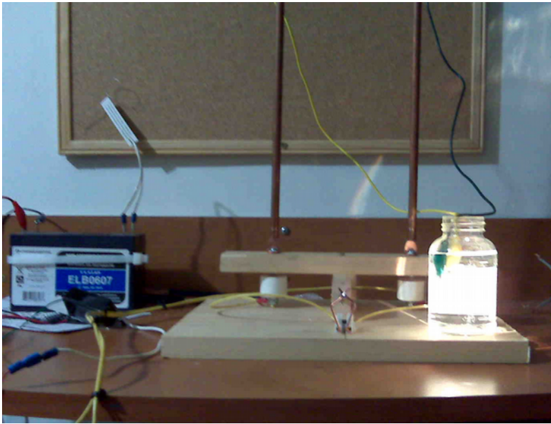
Hairpin circuit with light submerged in water
