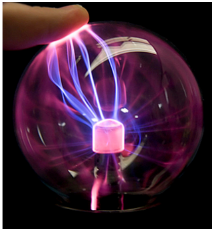
Plasma Ball
