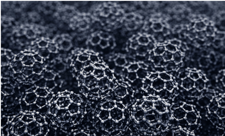
Buckyballs
