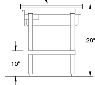
Heavy Gauge S/S Table Top with Countertop Edge SIDE VIEW
