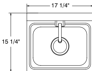
TOP VIEW for 7-PS-61, 7-PS-81 & 7-PS-91
