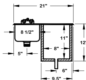
ELEVATION VIEW
