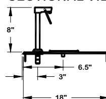
SECTIONAL VIEW
