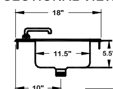
SECTIONAL VIEW
