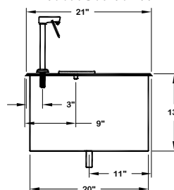
ELEVATION VIEW
