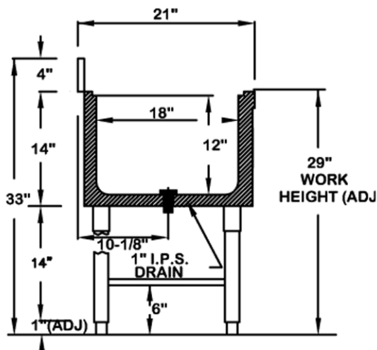
Sectional View
