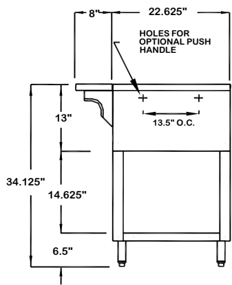
SECTIONAL VIEW
