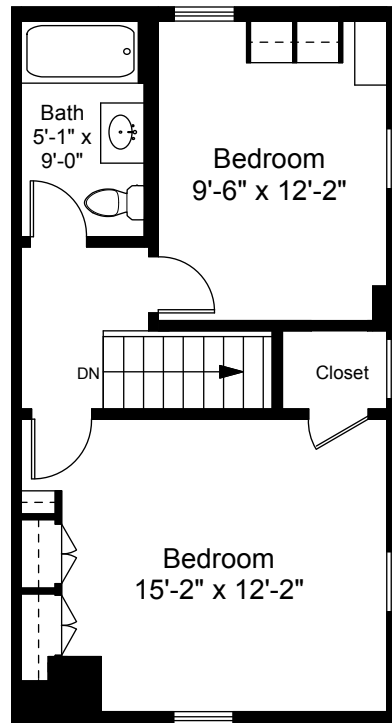
Second Floor Plan Ceiling Height = 7'-1"
