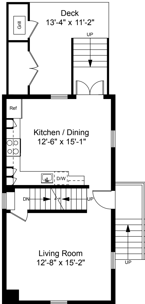
First Floor Plan Ceiling Height = 7'-8"
