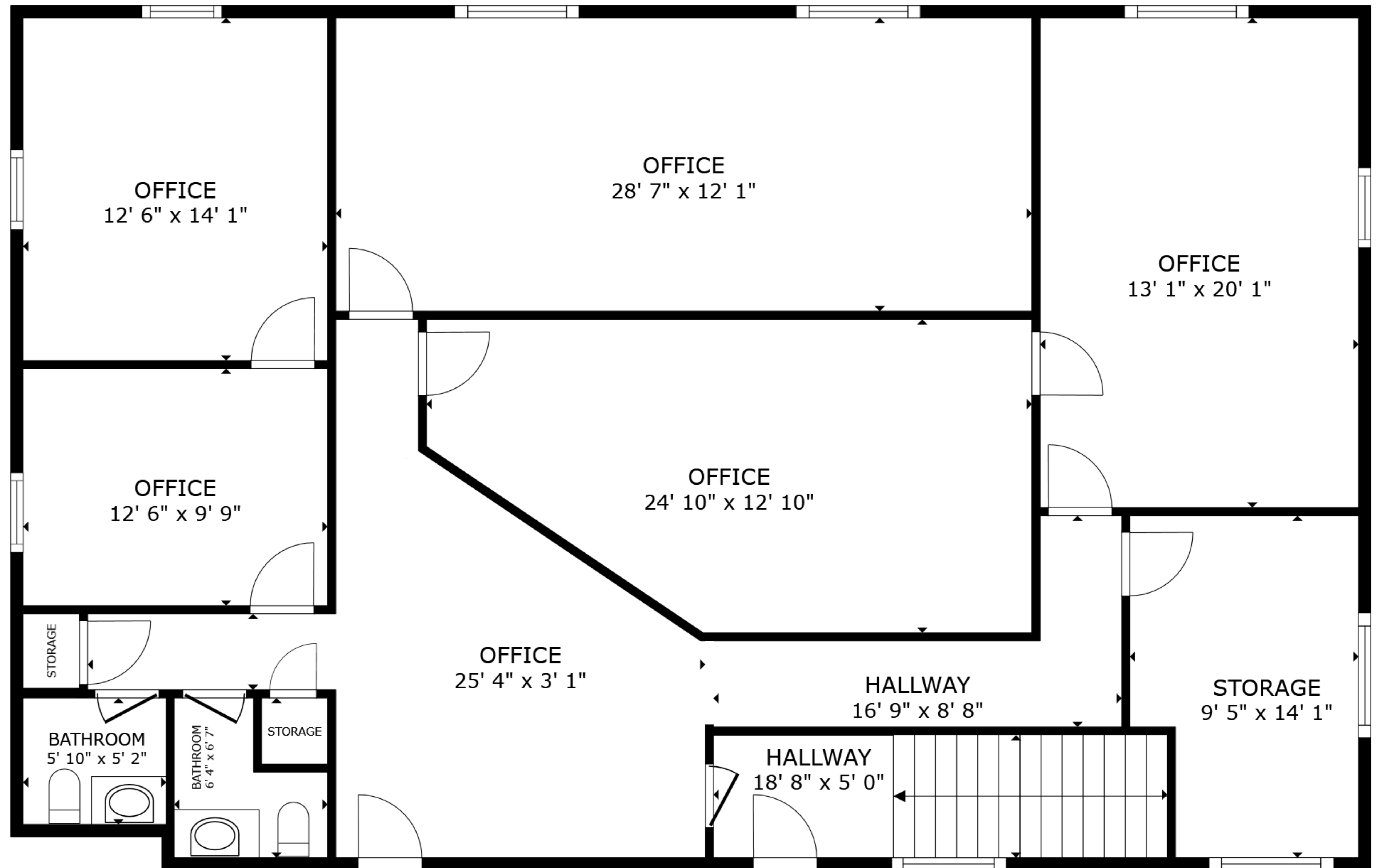
FLOOR 2
