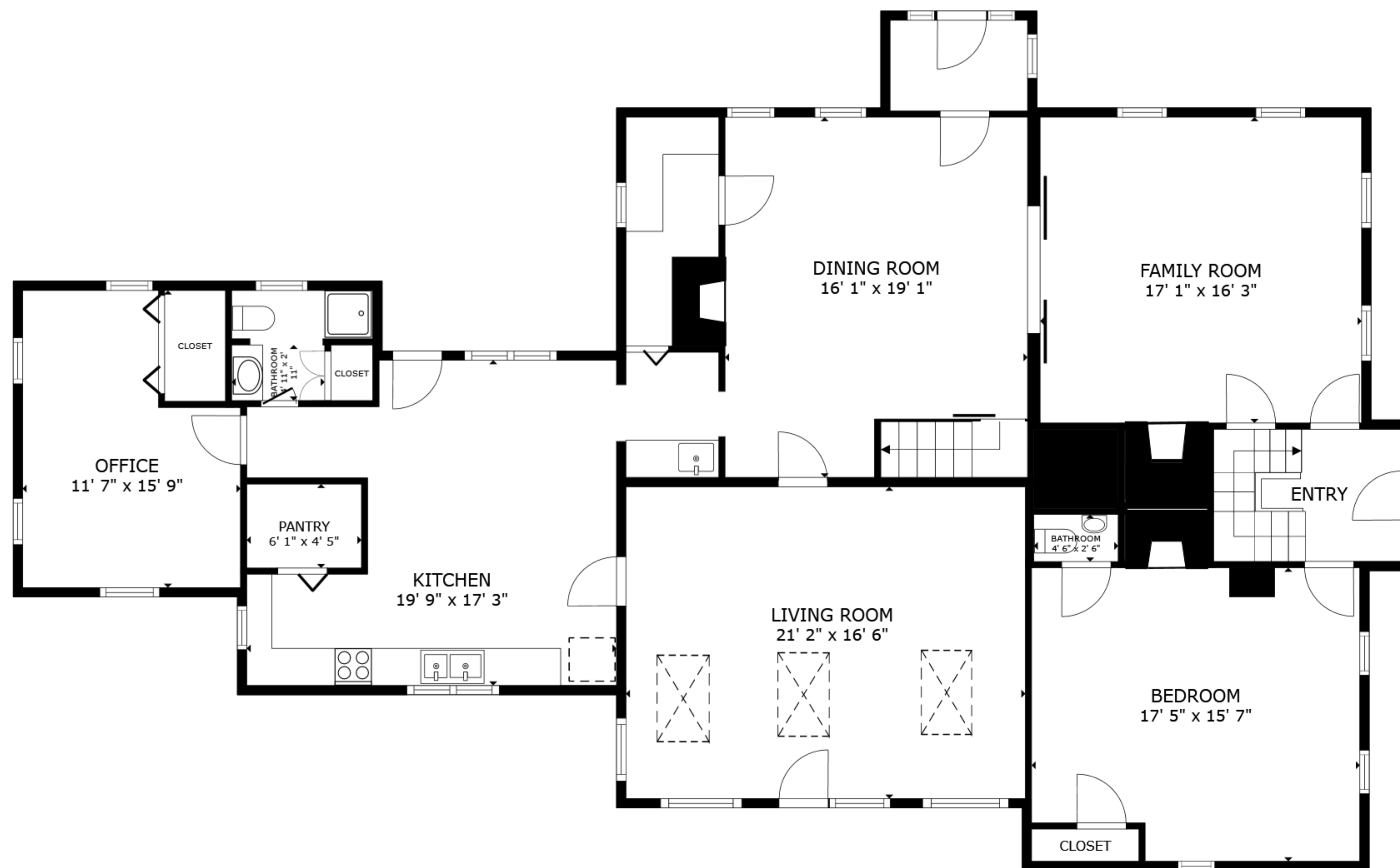
FLOOR 1
