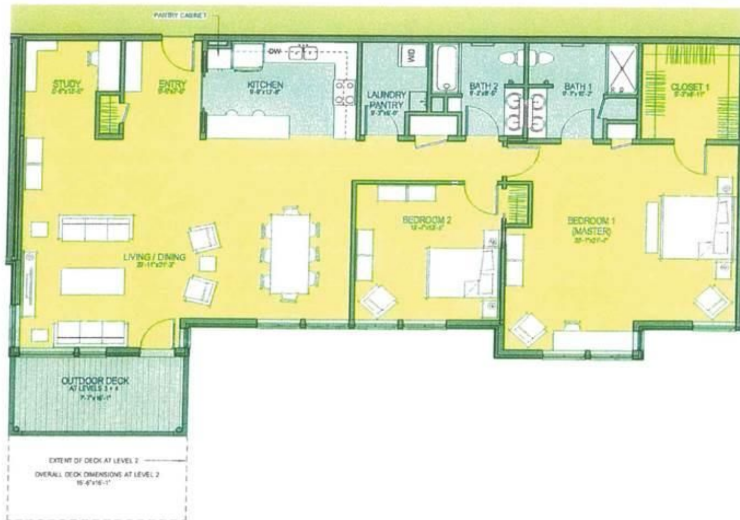
Unit Type E - Third Level AREA: 2040 SF
