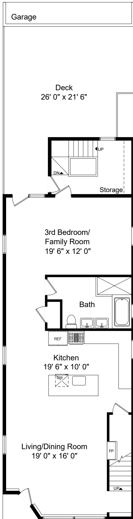
FIRST FLOOR
