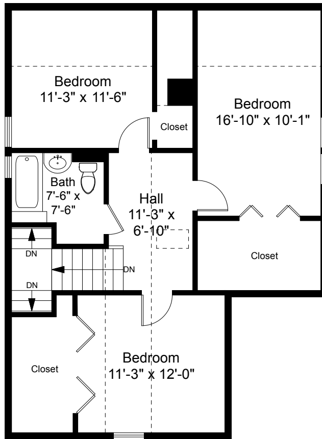
Second Floor Plan Ceiling Height = 7'-5"
