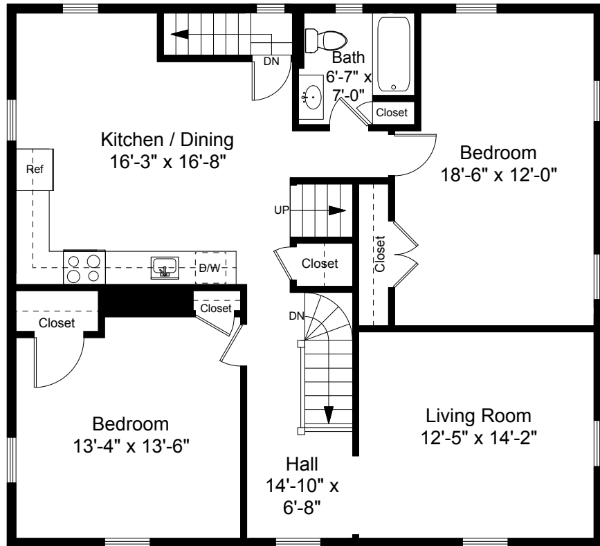
Second Floor Plan Ceiling Height = 7'-10"
