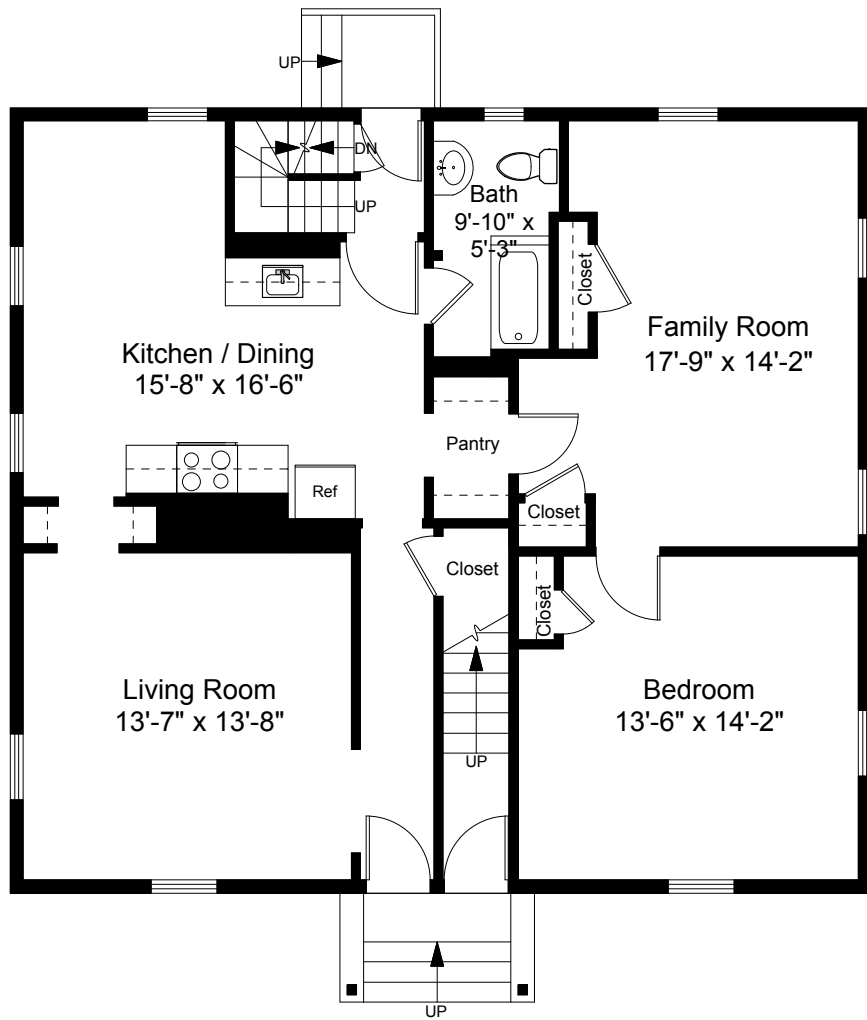
First Floor Plan Ceiling Height = 8'-6"
