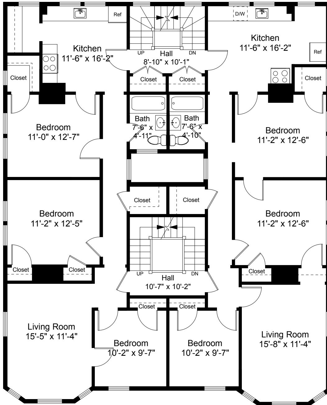
Second Floor Plan Ceiling Height = 9'-0"
