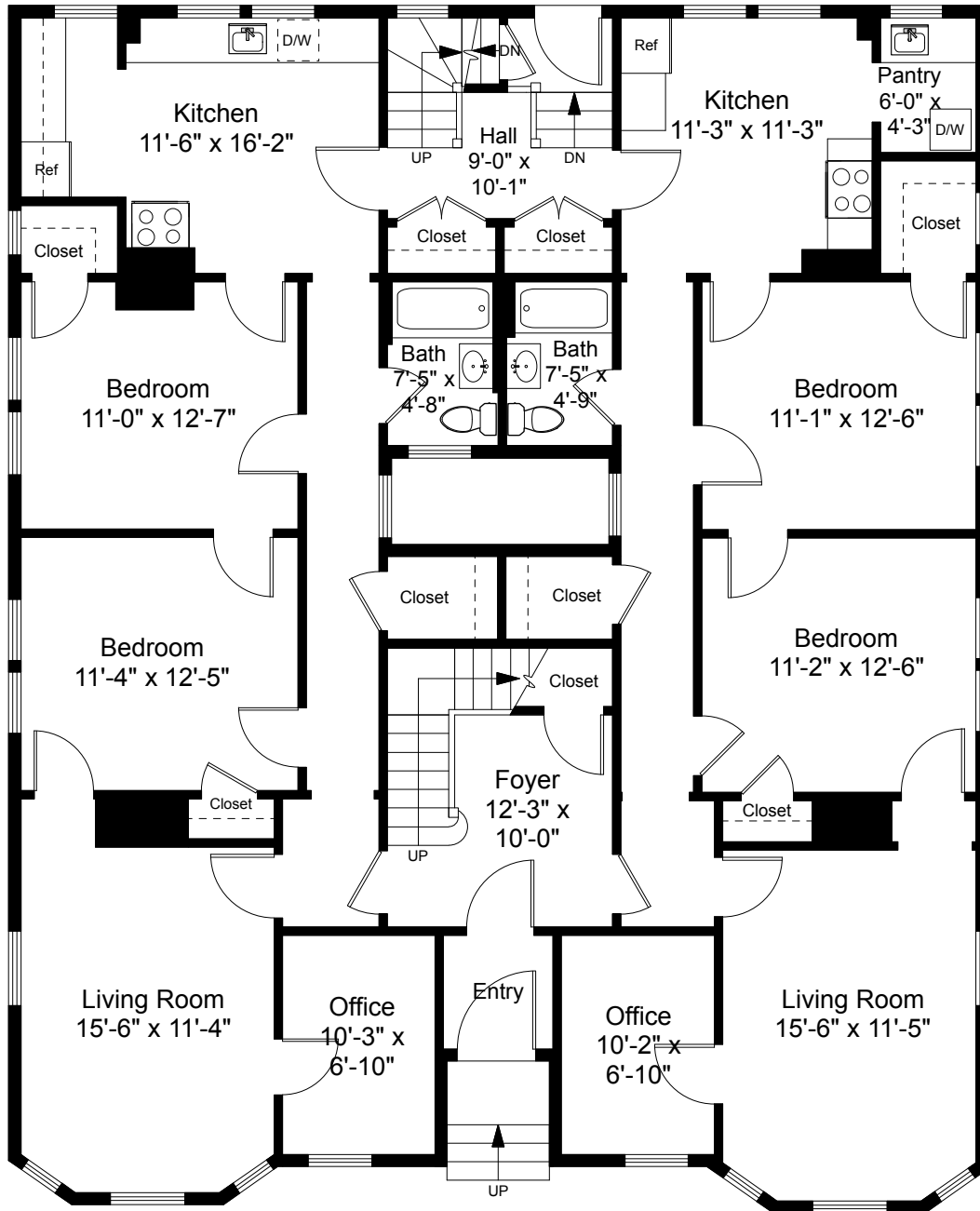
First Floor Plan Ceiling Height = 9'-6"
