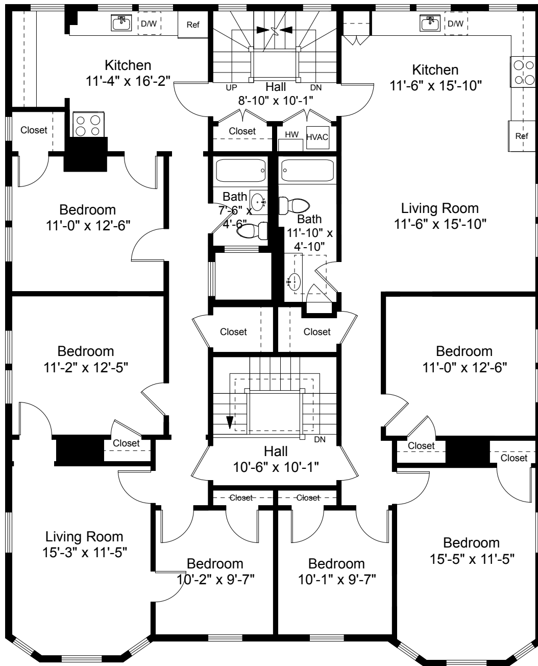
Third Floor Plan Ceiling Height = 9'-0"
