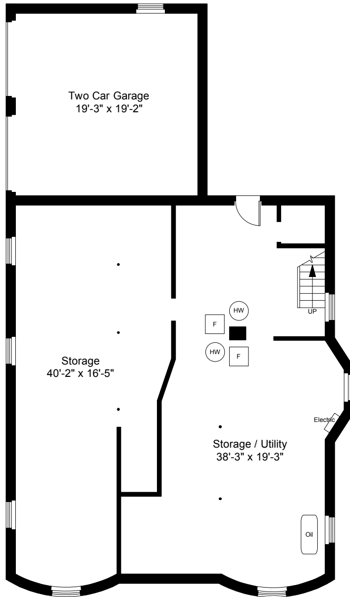
Basement Plan Ceiling Height = 7'-9"
