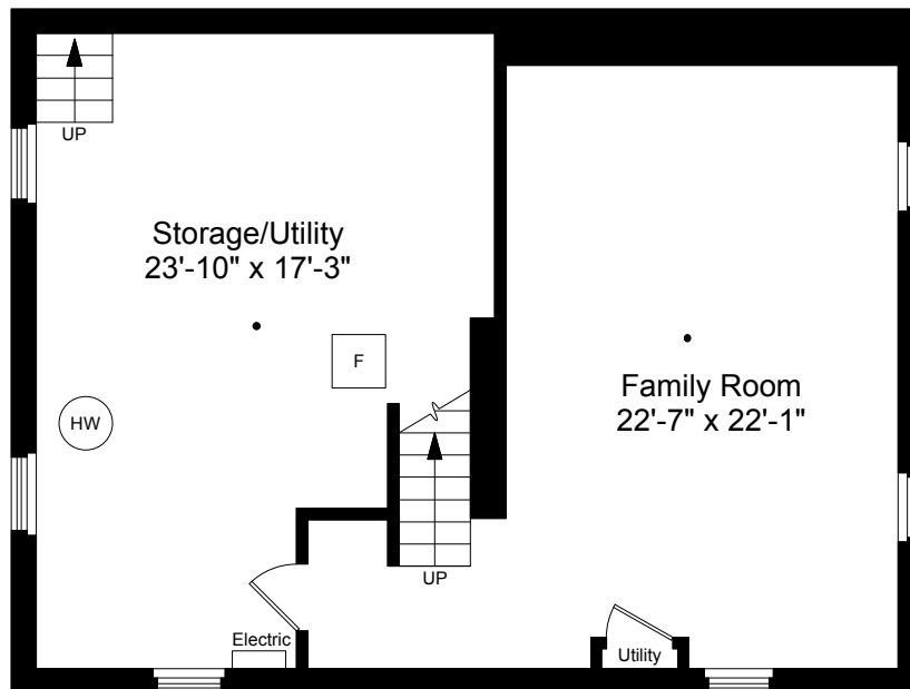
Lower Level Plan Ceiling Height = 6'-10"
