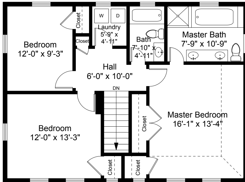
Second Floor Plan Ceiling Height = 7'-8"
