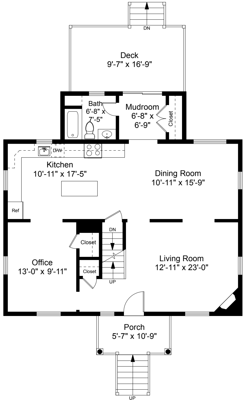
First Floor Plan Ceiling Height = 7'-8"
