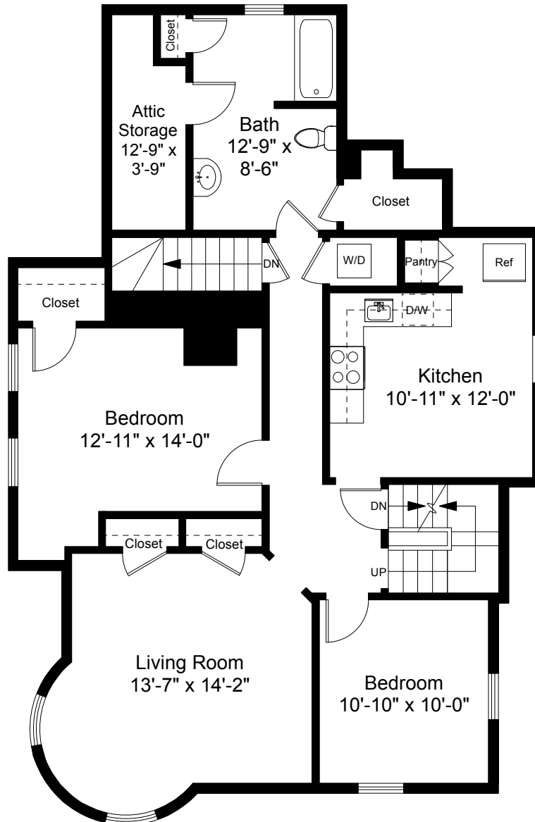
Second Floor Plan Ceiling Height = 9'-1"
