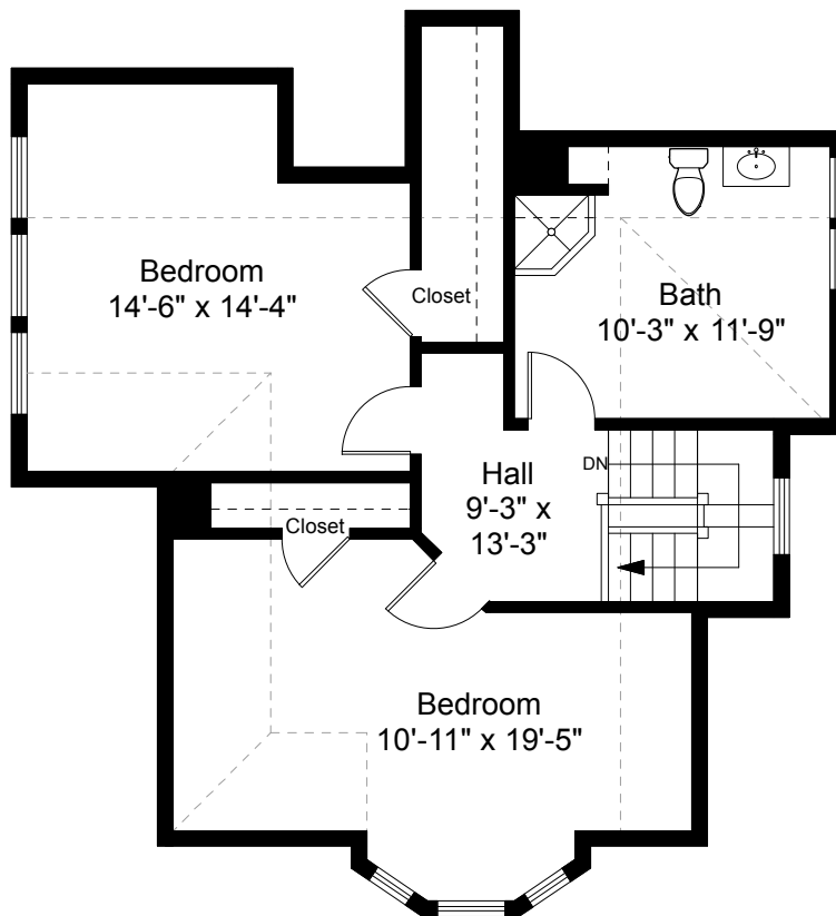
Third Floor Plan Ceiling Height = 7'-6"
