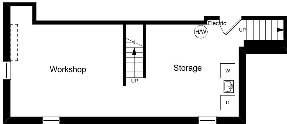
Basement Plan
