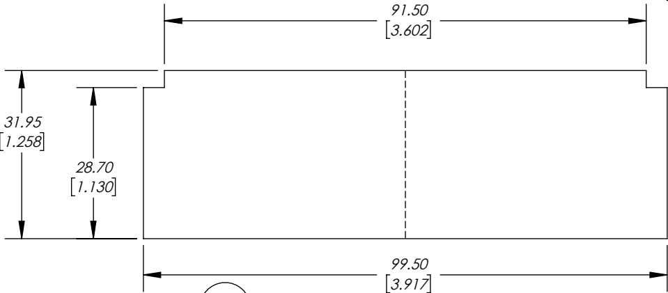
B1 MOUNTING PANEL CUTOUT
