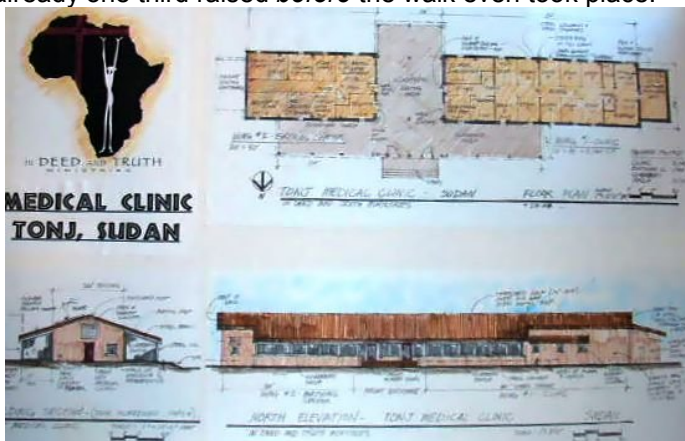
Tonj Medical Clinic Plans
