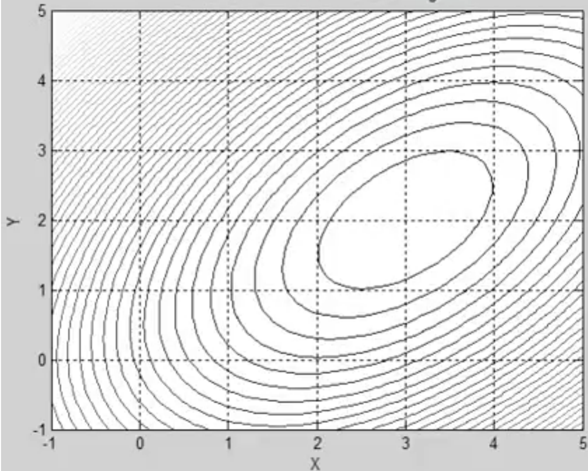
Contour Plot with Nedler Mead Triangles
