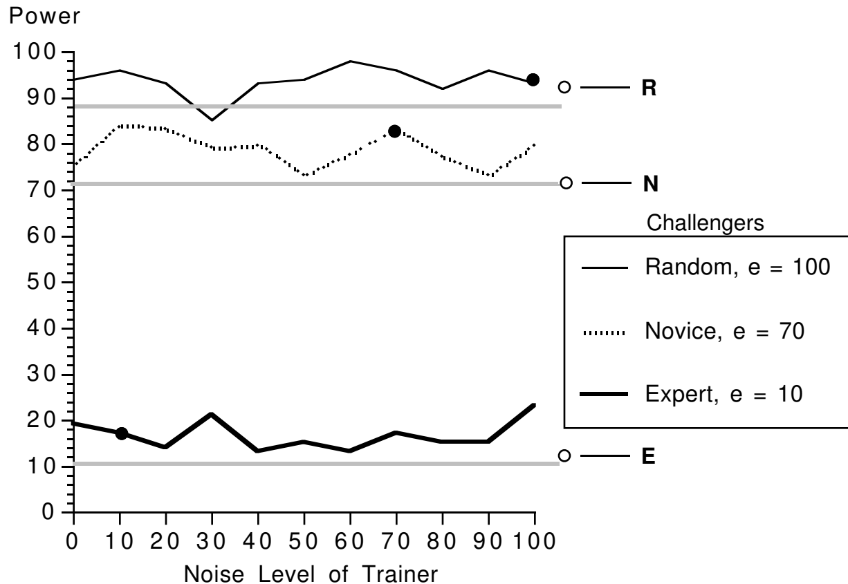
Figure 5: Power at tic-tac-toe measured against three different challengers after training. Training experiences have a noise level ranging from 0 to 100%. Points emphasized by black circles measure performance against a challenger exactly like the trainer. White circles labeled with letters denote values for self-training. Horizontal gray lines indicate the 95% confidence lower bound for maximal power.
