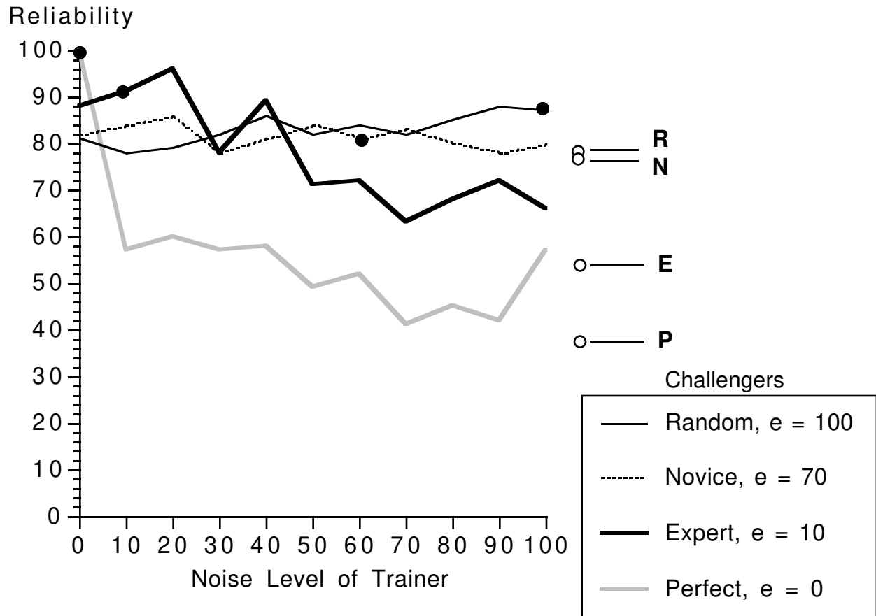
Figure 6: Reliability at lose tic-tac-toe measured against four different challengers after training. Training experiences have a noise level ranging from 0 to 100%. Points emphasized by black circles measure performance against a challenger exactly like the trainer. White circles labeled with letters denote values for self-training.
