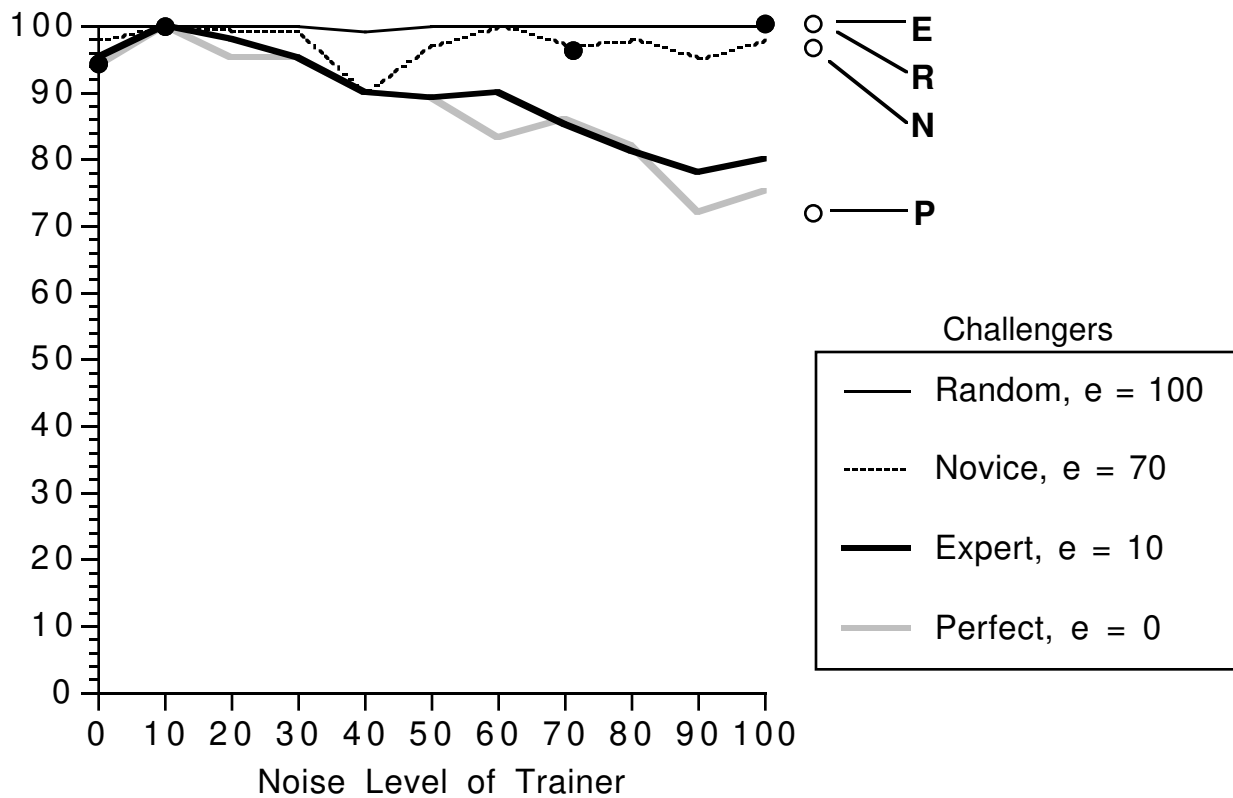
Figure 4: Reliability at tic-tac-toe measured against four different challengers after training. Training experiences have a noise level ranging from 0 to 100%. Points emphasized by black circles measure performance against a challenger exactly like the trainer. White circles labeled with letters denote values for self-training.
