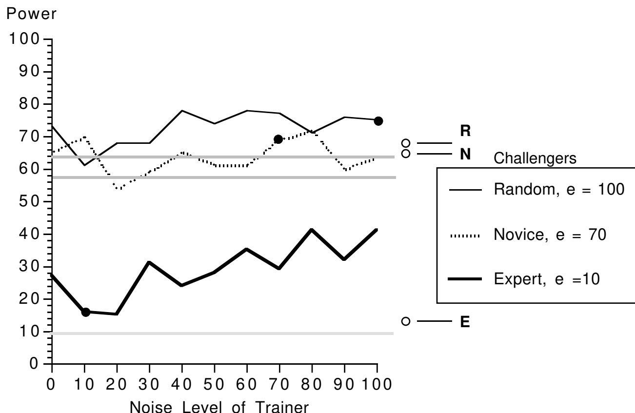
Figure 7: Power at lose tic-tac-toe measured against three different challengers after training. Training experiences have a noise level ranging from 0 to 100%. Points emphasized by black circles measure performance against a challenger exactly like the trainer. White circles labeled with letters denote values for self-training. Horizontal gray lines indicate the 95% confidence lower bound for maximal power.
