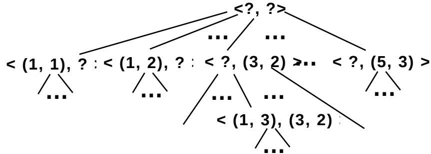
Figure 2. Part of the carousel problem state space.
