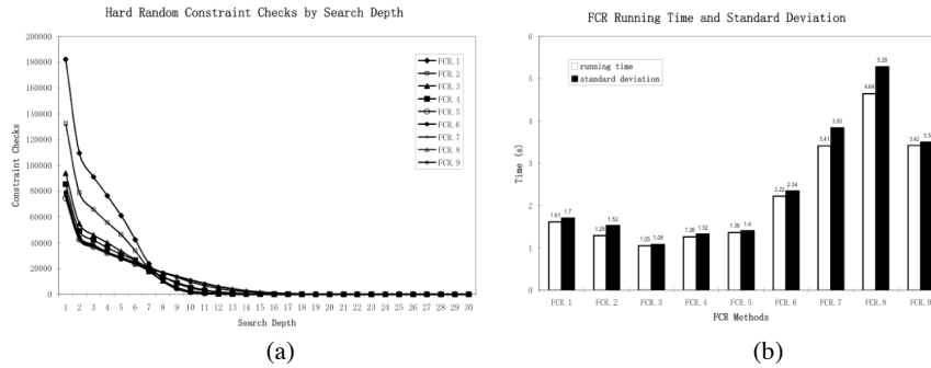
Figure 1: (a) The number of constraint checks with Min Domain/Degree on 100 random problems in \langle 30, 8, 0.26, 0.34 \rangle for FCR propagation with r = .1, .2, \dots, .9 . (b) Running time average and standard deviation for these runs. Note that the best time appears to be for r = 0.3 .
