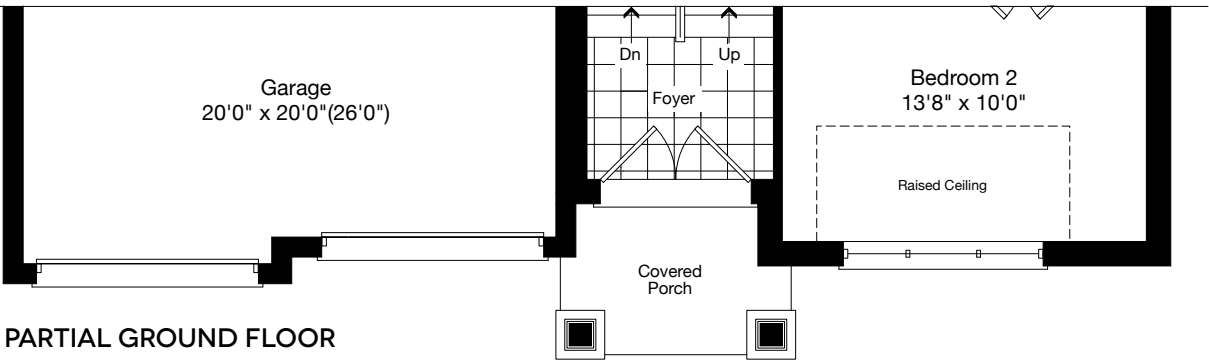
PARTIAL GROUND FLOOR ELEVATION B
