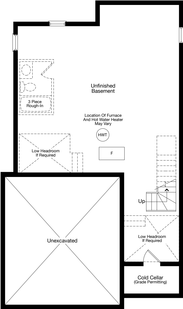
BASEMENT ELEVATION A & B
