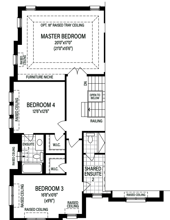
Partial Second Floor Elevation B
