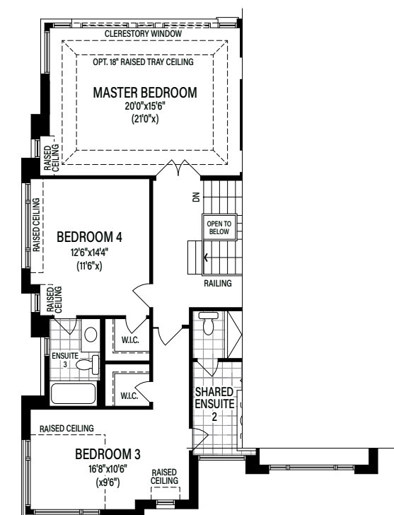
Partial Second Floor Elevation C
