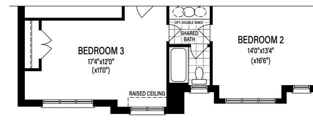
Partial Second Floor Elevation B
